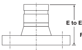
Figure 341 Flange Adapter
