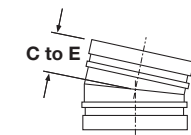
FIGURE 313 FABRICATED 11-1/4° ELBOW (SEGMENT WELDED)
