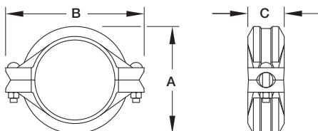
Figure 577 Rigid Coupling
