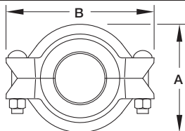
Figure 716 Flexible Reducing Coupling 1 of 2
