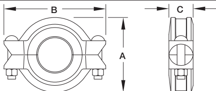
Figure 716 Flexible Reducing Coupling 2 of 2
