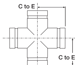
FIGURE 327 FABRICATED CROSS (SEGMENT WELDED)
