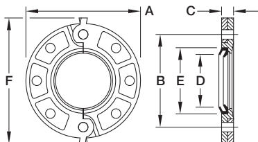
FIGURE 71 PN16 (METRIC)
