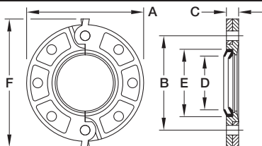
Figure 71 Flange Adapter
